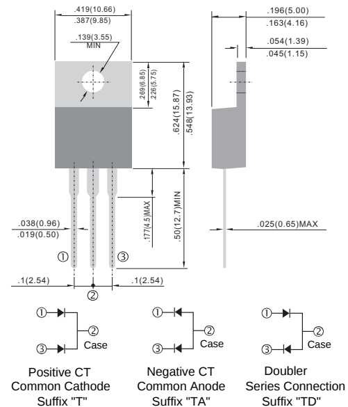
TO-220AB
