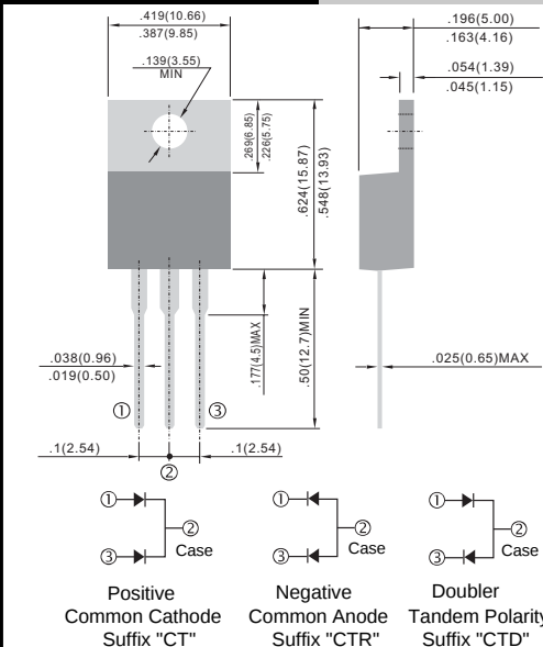
TO-220AB
