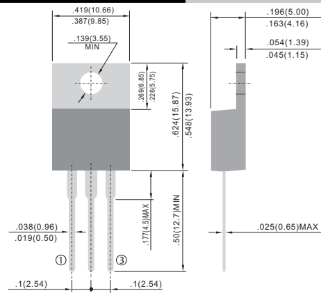
TO-220AB
