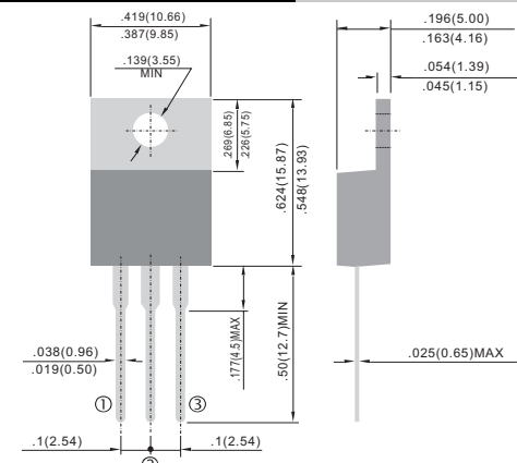
TO-220AB
