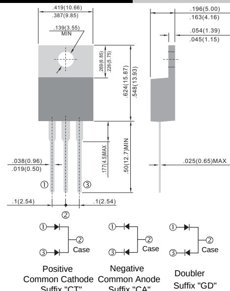
TO-220AB
