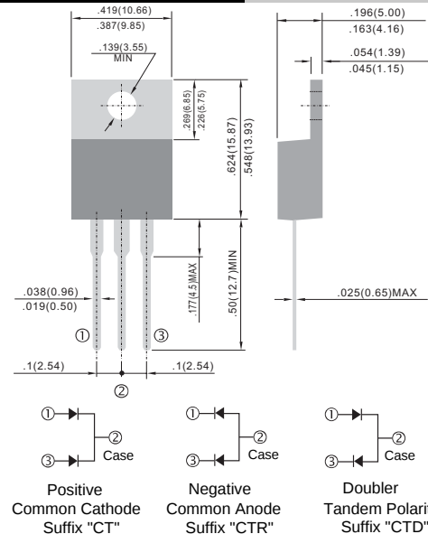
TO-220AB
