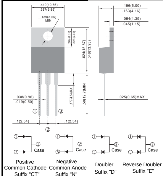
TO-220AB
