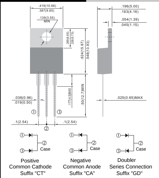
TO-220AB
